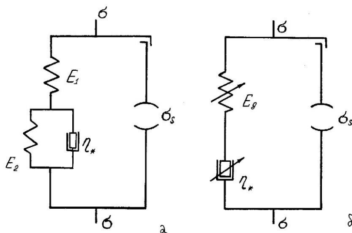
Fig. 1. Rheological models of cutting objects:
