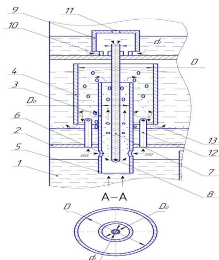
Figure 1. Intensified bubbling extractor
